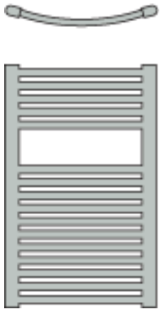
SB50/75H Height 750 mm Width 500 mm Centres 460 mm Output 266 watts
