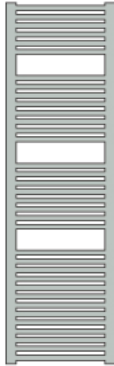
SB50/165H Height 1650 mm Width 500 mm Centres 460 mm Output 554 watts
