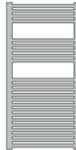
SB60/118H Height 1118 mm Width 600 mm Centres 560 mm Output 450 watts
