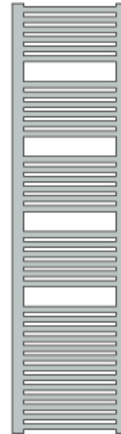
S50/165H Height 1650 mm Width 500 mm Centres 460 mm Output 554 watts HE & E 350 watts
