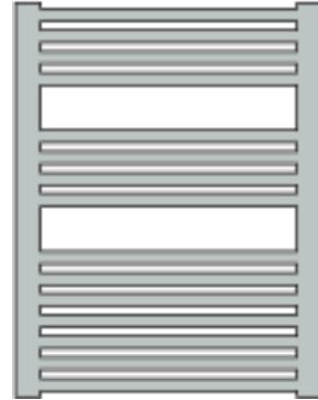
S60/75H Height 750 mm Width 600 mm Centres 560 mm Output 311 watts HE & E 150 watts
