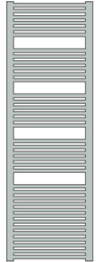
S60/165H Height 1650 mm Width 600 mm Centres 560 mm Output 647 watts HE & E 450 watts
