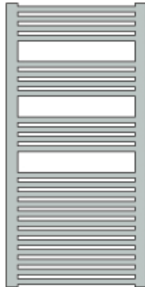
S60/118H Height 1118 mm Width 600 mm Centres 560 mm Output 450 watts HE & E 350 watts
