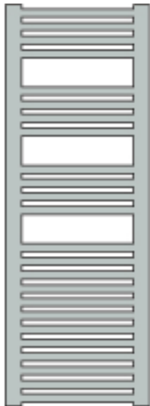
S45/118H Height 1118 mm Width 450 mm Centres 410 mm Output 354 watts HE & E 250 watts
