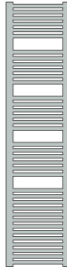
S45/165H Height 1650 mm Width 450 mm Centres 410 mm Output 531 watts HE & E 350 watts
