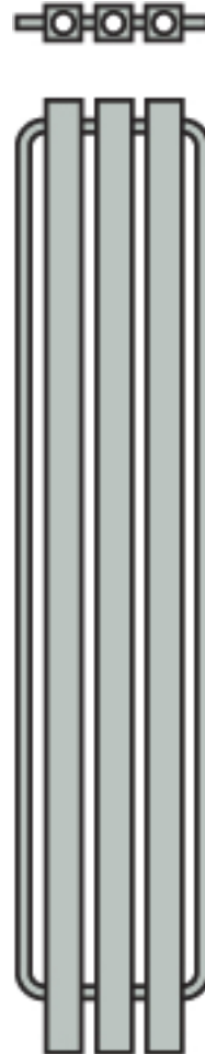
H1800/3 Height 1800 mm Width 350 mm Depth 70 mm Output 1835 watts
