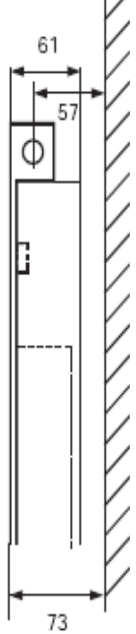
Bracket / projection / connection Detail
