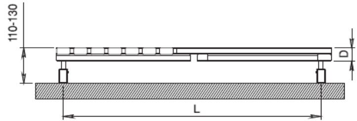
Connections Detail
