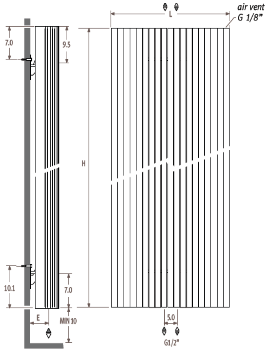
Arco Technical Detail : RC/PW/01.11
